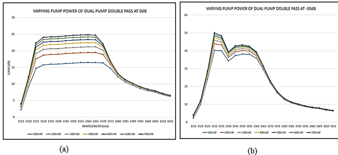
Fig. 9. Graph of Gain Performance for Dual Pump Double Pass with Varying Pump Power at (a) 0 dB (b) -30dB
