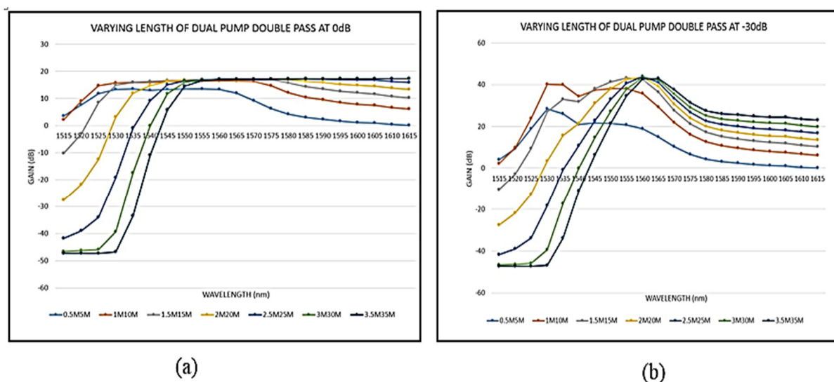
Fig. 7. Graph of Gain Performance for Dual Pump Double Pass with Varying EDFA Length at (a) 0 dB (b) -30 dB
