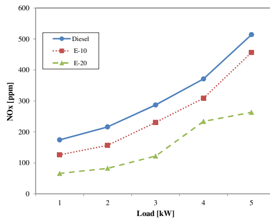
Fig. 5. The amount of NOx measurement for different fuel at varying load conditions
