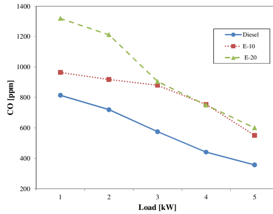
Fig. 4. The amount of CO for different fuel at varying load conditions
