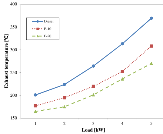
Fig. 3. Exhaust temperature for different fuel at varying load conditions
