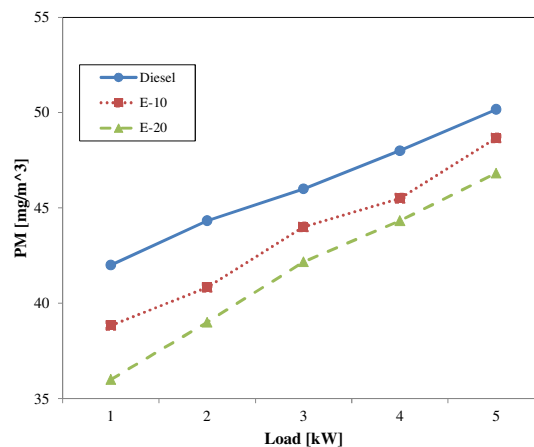
Fig. 2. PM measurement for different fuel at varying load conditions
