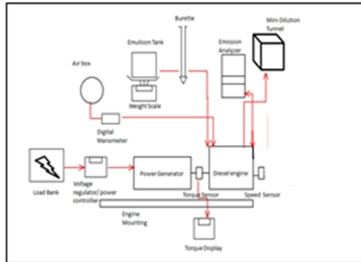
Fig. 1. The schematic of engine testing setup
