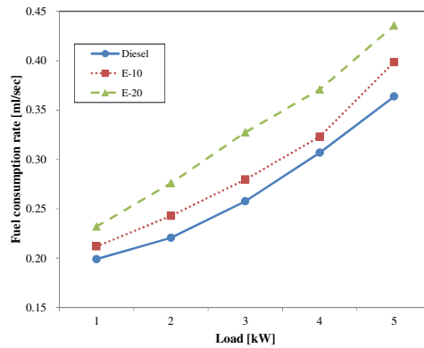
Fig. 6. Fuel consumption for different fuel at varying load conditions by considering the diesel and water as total fuel
