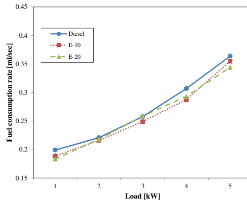
Fig. 7. Fuel consumption for different fuel at varying load conditions by considering the diesel as total
