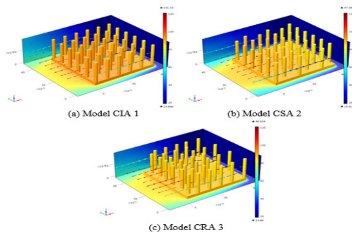
Figure 15: 3D circular pin fin heat sink models with different arrangement. Model CIA 1 (max temp: 101.03^{\circ}\text{C} ); (b) Model CSA 2 (max temp: 97.366^{\circ}\text{C} ); (c) Model CRA 3 (max temp: 96.904^{\circ}\text{C} )
