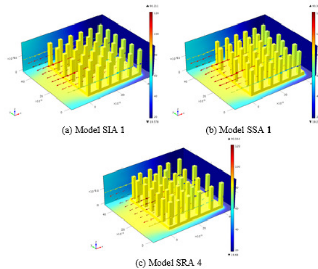
Figure 16: 3D square pin fin heat sink models with different arrangement. Model SIA 1 (max temp: 90.211^{\circ}\text{C} ); (b) Model SSA 1 (max temp: 90.399^{\circ}\text{C} ); (c) Model SRA 4 (max temp: 90.044^{\circ}\text{C} )
