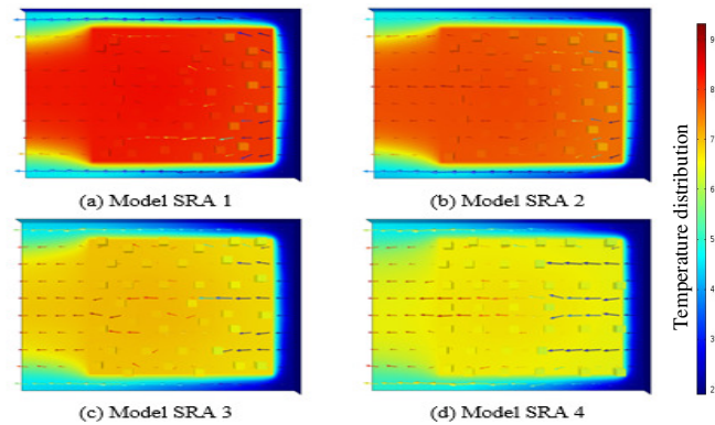
Figure 14: Top view plot of temperature and airflow for SRA of pin fin heat sink models. . (a) Model SRA 1 (max temp: 111.9^{\circ}\text{C} ); (b) Model SRA 2 (max temp: 106.01^{\circ}\text{C} ); (c) Model SRA 3 (max temp: 94.383^{\circ}\text{C} ); (d) Model SRA 4 (max temp: 90.044^{\circ}\text{C} )
