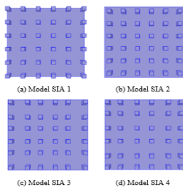
Figure 6: Top view of SIA pin fin model
