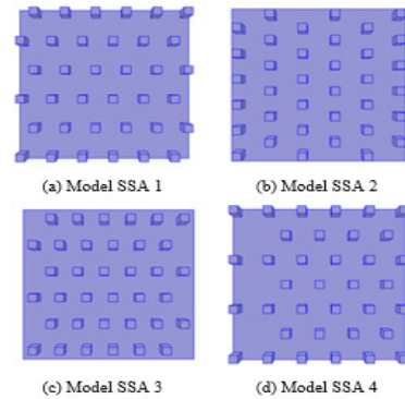
Figure 7: Top view of SSA pin fin model
