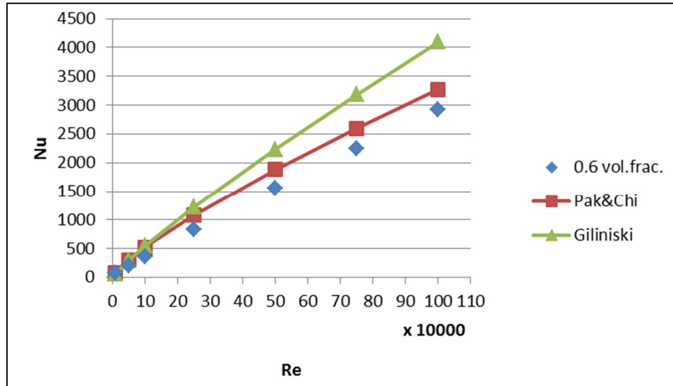
Figure 3: Comparison of computed results with the correlations at 0.6% volume fraction
