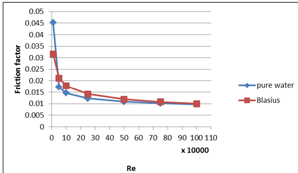
Figure 5: Comparison of computed results of friction factor of pure water with the correlation of Blasius
