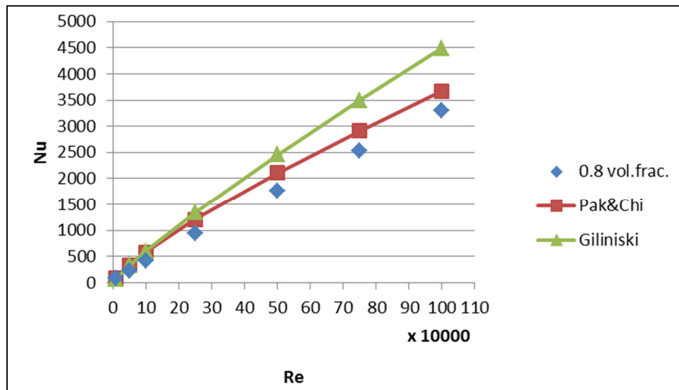
Figure 4: Comparison of computed results with the correlations at 0.8% volume fraction
