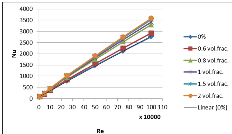
Figure 2: Effect of nanofluid concentrations and Reynolds number on average Nusselt number.
