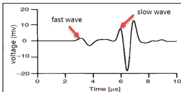
Fig. 4. Observable fast and slow wave in time domain [39]
