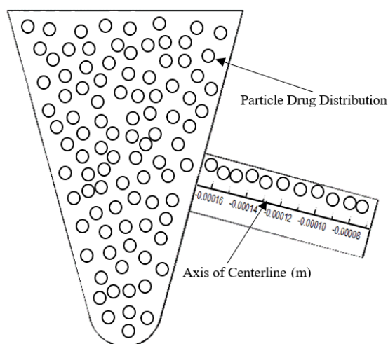
Fig. 4. Axis of centerline inside the actuator nozzle
