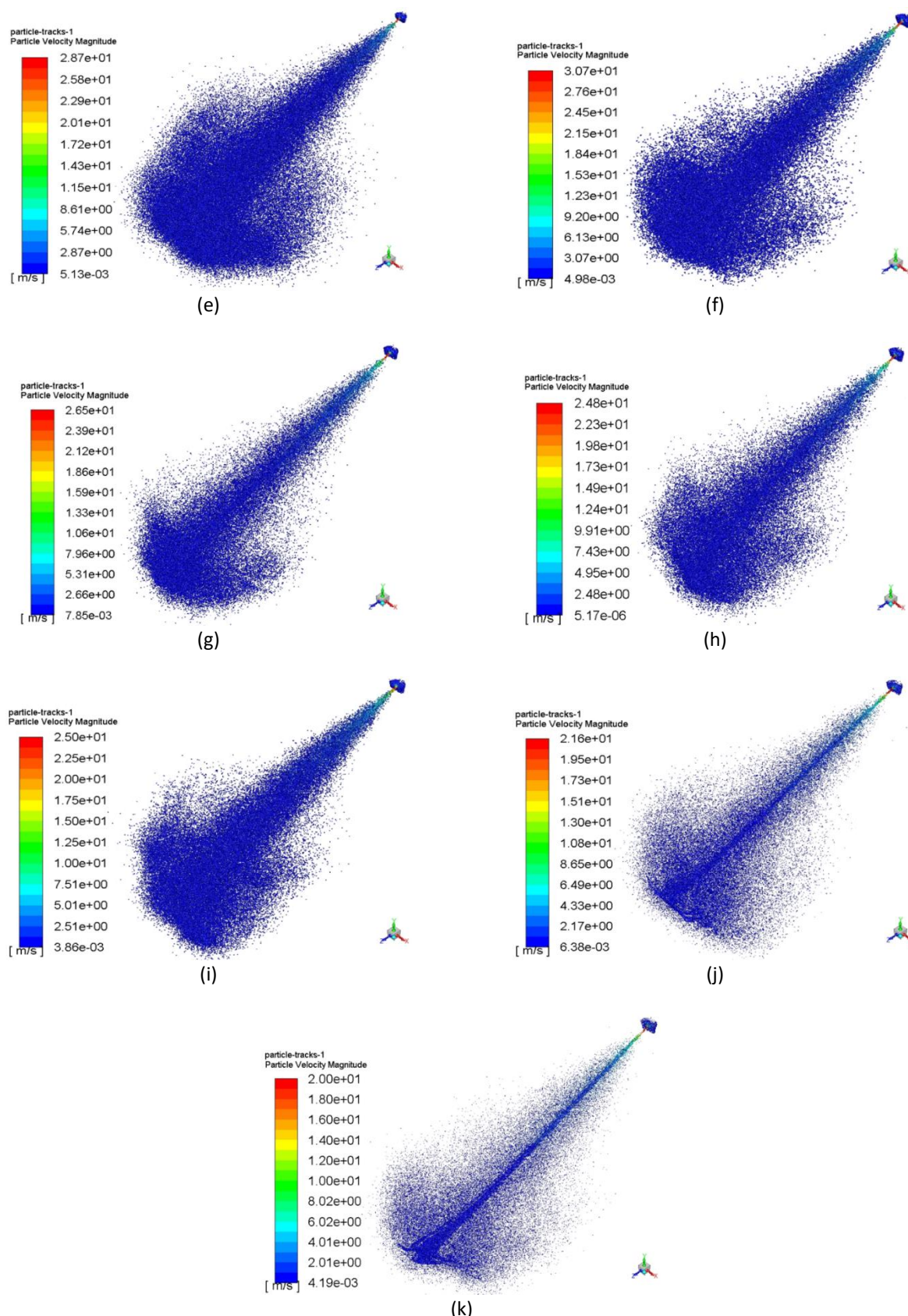
Fig. 6. Particle velocity magnitude on different orifice diameter inside the actuator nozzle; (a) 0.39mm orifice diameter, (b) 0.41mm orifice diameter, (c) 0.43mm orifice diameter, (d) 0.45mm orifice diameter, (e) 0.47mm orifice diameter, (f) 0.49mm orifice diameter, (g) 0.51mm orifice diameter, (h) 0.53mm orifice diameter, (i) 0.55mm orifice diameter, (j) 0.57mm orifice diameter, (k) 0.59mm orifice diameter
