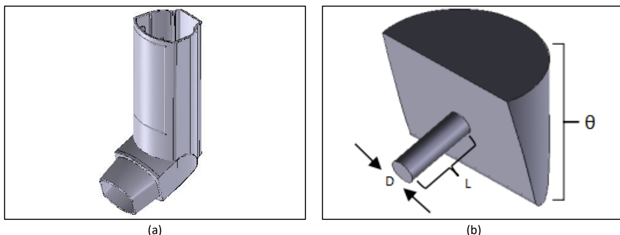
Fig. 2. Geometrical modelling of pMDI inhaler device (a) 3D design of pMDI inhaler using Solidwork 2016, (b) Schematic diagram of internal parts in the actuator nozzle
