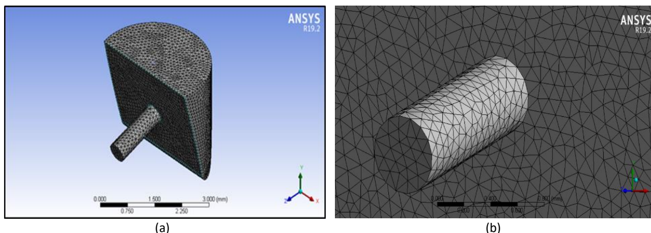
Fig. 3. Meshing process for internal parts in the actuator nozzle (a) Meshed model of the nozzle (b) Details view for the orifice diameter in the actuator nozzle
