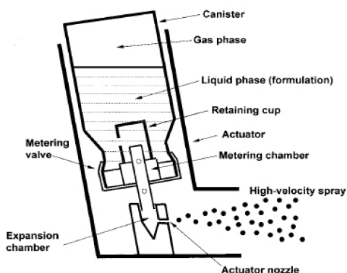
Fig. 1. pMDI schematic cross-section [10]
