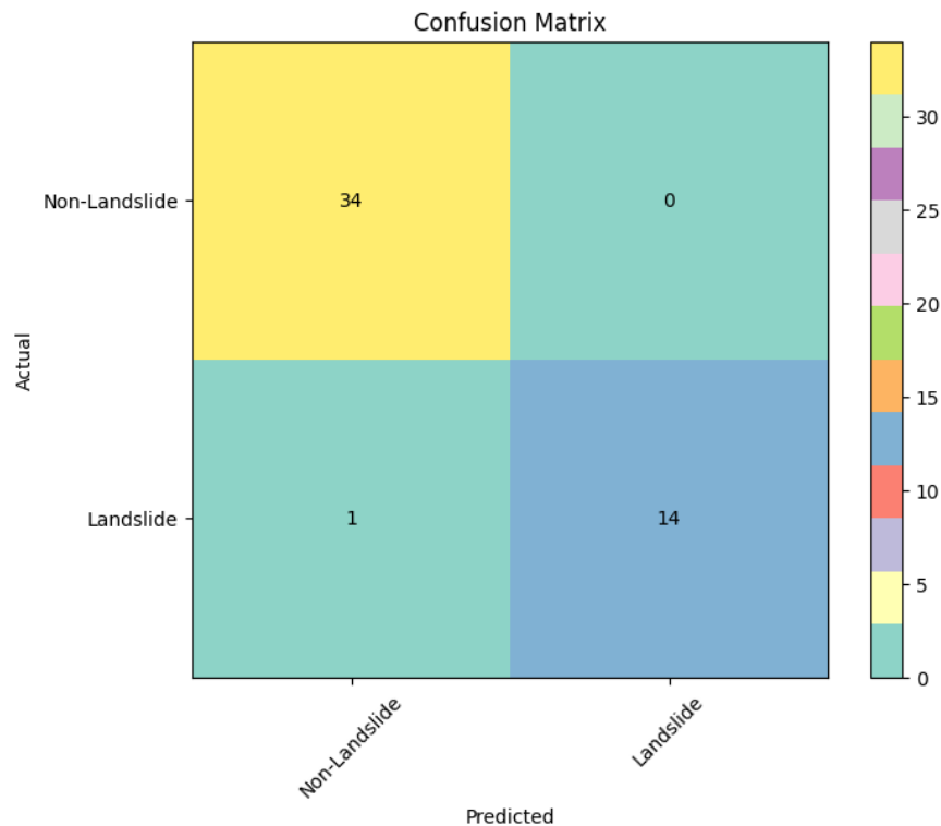
Fig. 4. Prediction outcome
