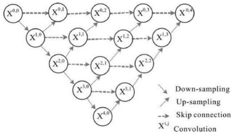
Fig. 5. The architecture of U-Net+ network
