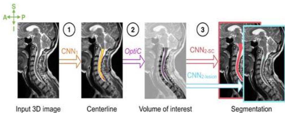
Fig. 3. Automatic segmentation framework
